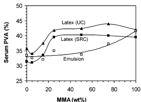
Figure 10. Amount of serum PVA in latexes and miniemulsions as a function of monomer composition; UC = ultracentrifugation, diluted to ~10 wt % solids content; SRC = the serum replacement cell, ~20 wt % (original solids content); lines drawn for visualization purposes only.
